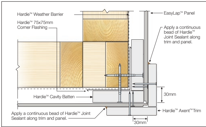
FIGURE 22 TRIM CORNER OPTION - CAVITY BATTEN
