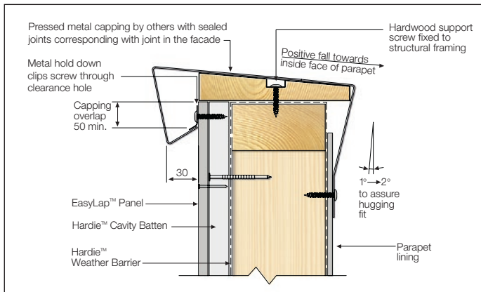
FIGURE 19 PARAPET CAPPING DETAIL
