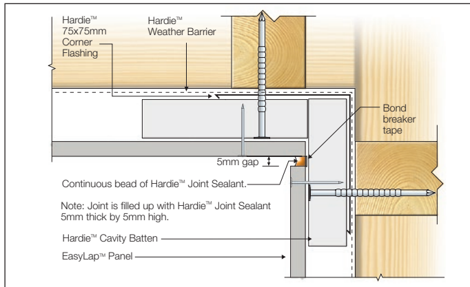
FIGURE 24 SEALANT FILL OPTION - CAVITY BATTEN
