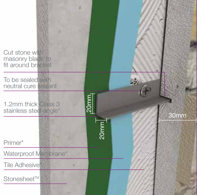
Figure 5 Example of Installation of angle bracket on Innova Stonesheet™- screw fixed to stud
