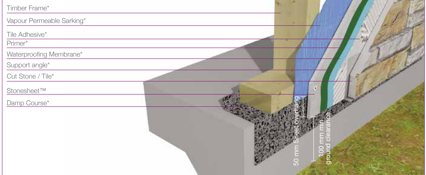
Figure 11 Ground Clearance
